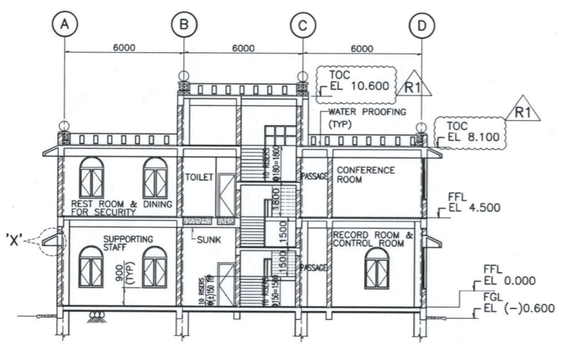
SECTION 2-2 SCALE 1:100
