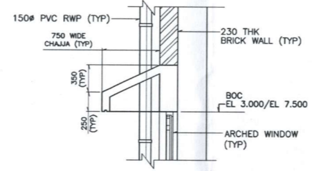
DETAIL 'X' SCALE 1:25
